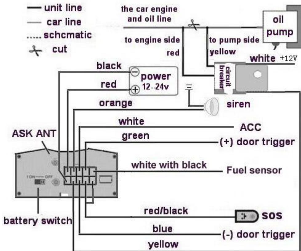
Wiring diagram
